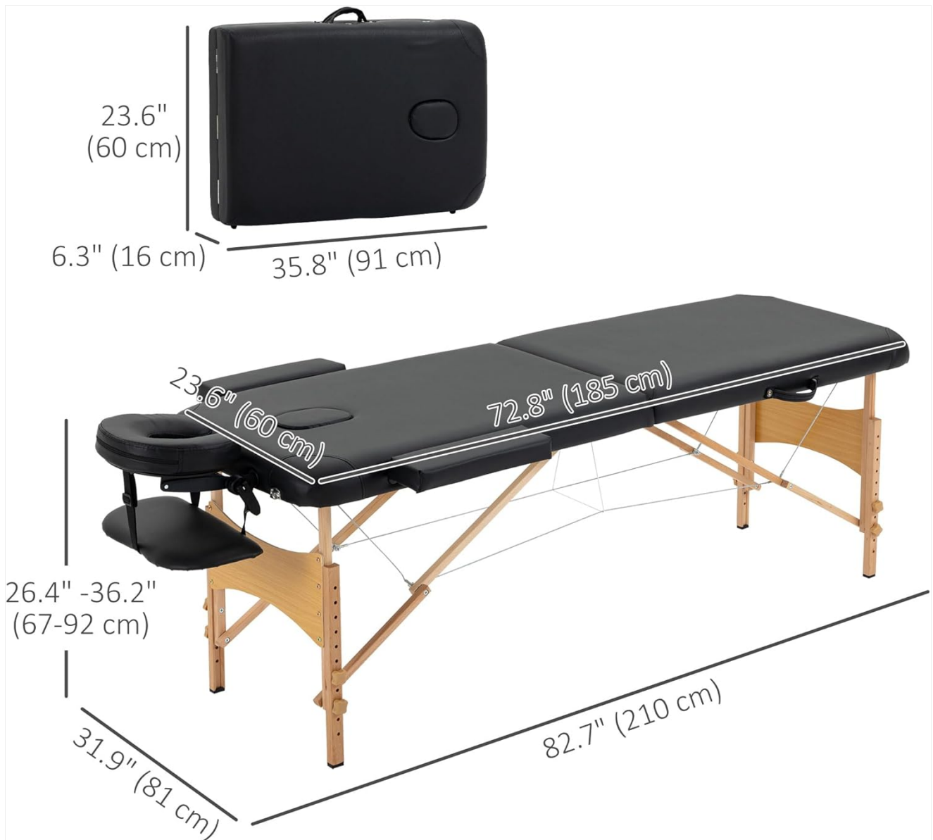
Image: A detailed diagram illustrating the overall dimensions of the massage table when set up and when folded for storage.
