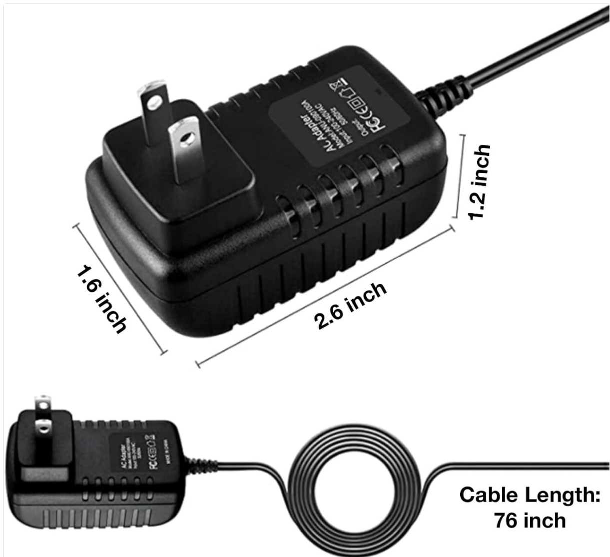
Image: Diagram illustrating the dimensions of the LKPower 6V AC Adapter Charger, including its length, width, height, and cable length.
