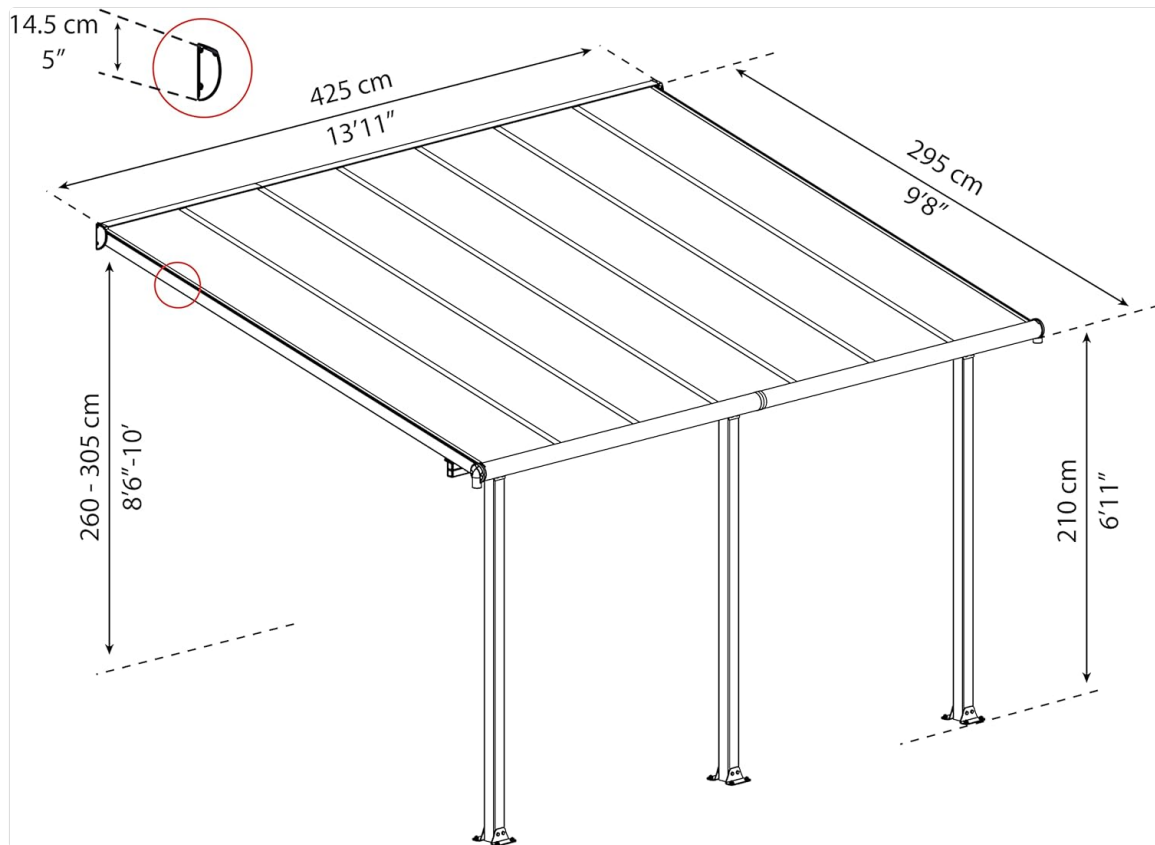
Figure 3: Side view of the Olympia Patio Cover, highlighting its lean-to design.
