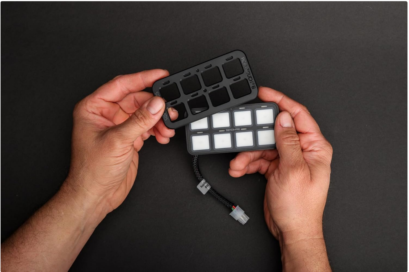
Figure 2: Close-up view of the 8-switch panel and its bezel, demonstrating how the panel fits into the mounting hardware.
