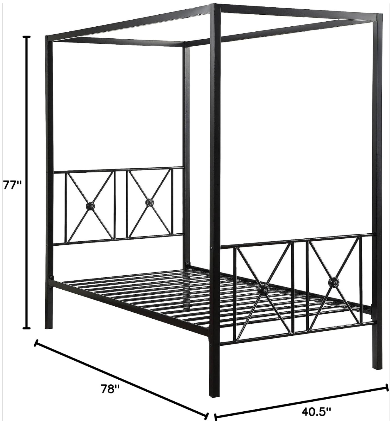
Figure 4.2: Detailed dimensions of the Homelegance Rapa Metal Canopy Bed.
