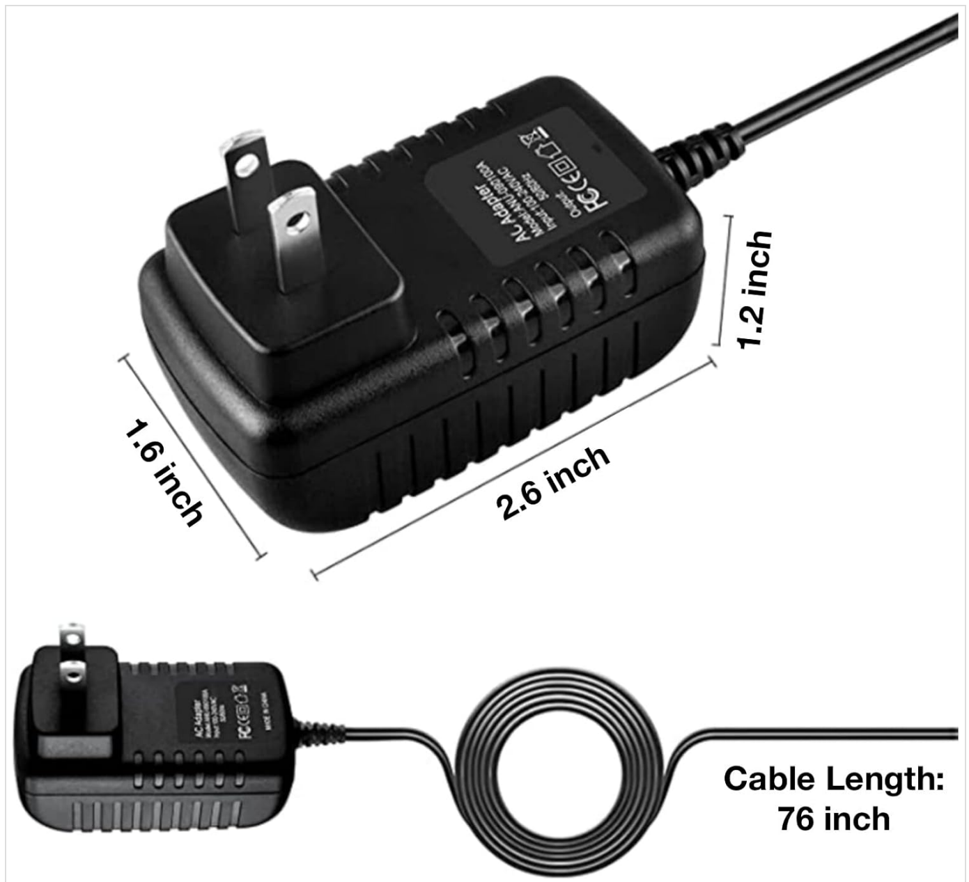
Image: Diagram illustrating the dimensions of the LKPower AC Adapter. The adapter measures approximately 2.6 inches in length, 1.6 inches in width, and 1.2 inches in height. The cable length is approximately 76 inches.
