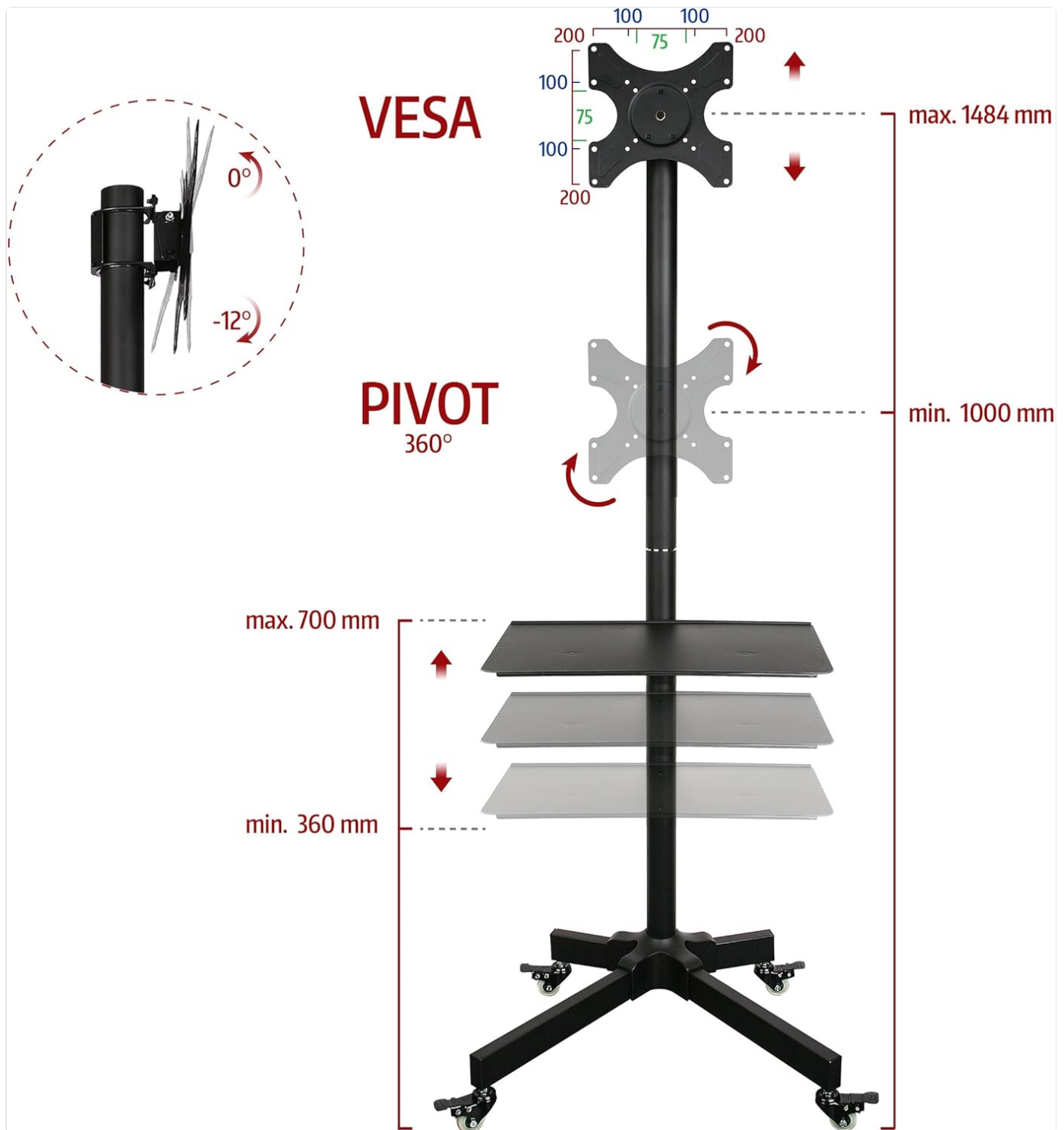
Figure 4.2: Diagram detailing VESA mounting patterns, 360° pivot, and adjustable height ranges for the TV and shelf.
