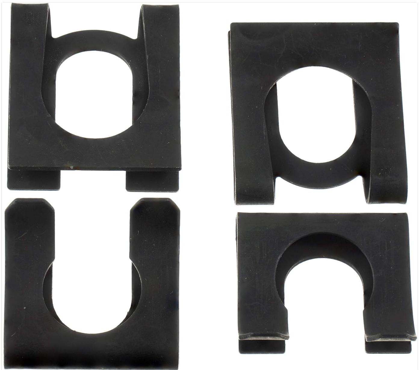
Figure 3.1: APDTY 24098 Brake Hydraulic Hose Line Retaining Clips. This image displays the four black metal clips included in the kit, showing their distinct shapes designed for securing brake lines.
