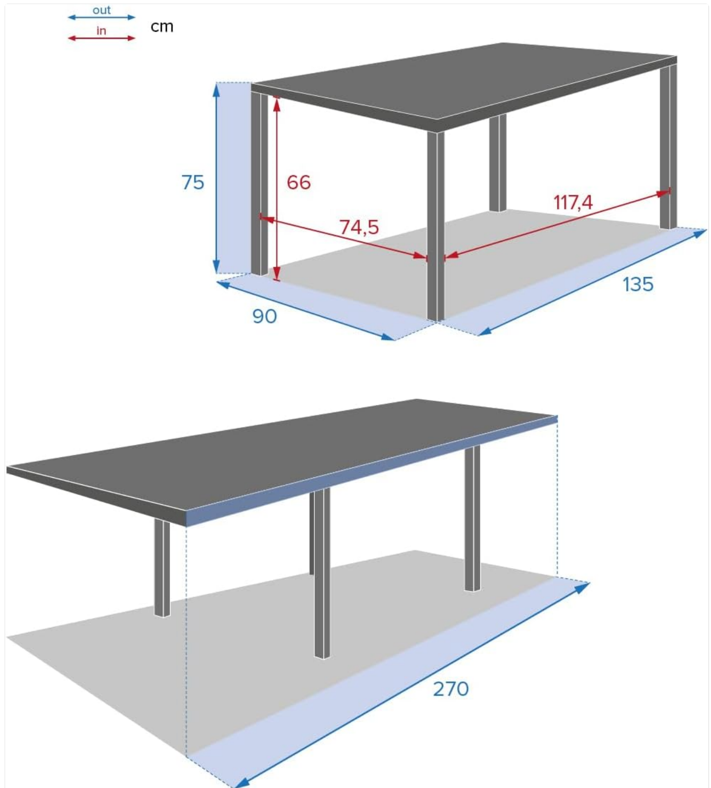
Image 5.1: Table with one extension leaf partially pulled out, showing the extension mechanism.
