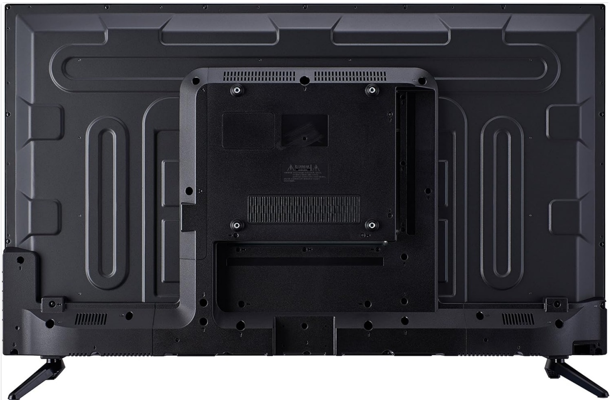
Figure 3.3: Back panel of the TV, illustrating the arrangement of input/output ports and the standard VESA mounting pattern.
