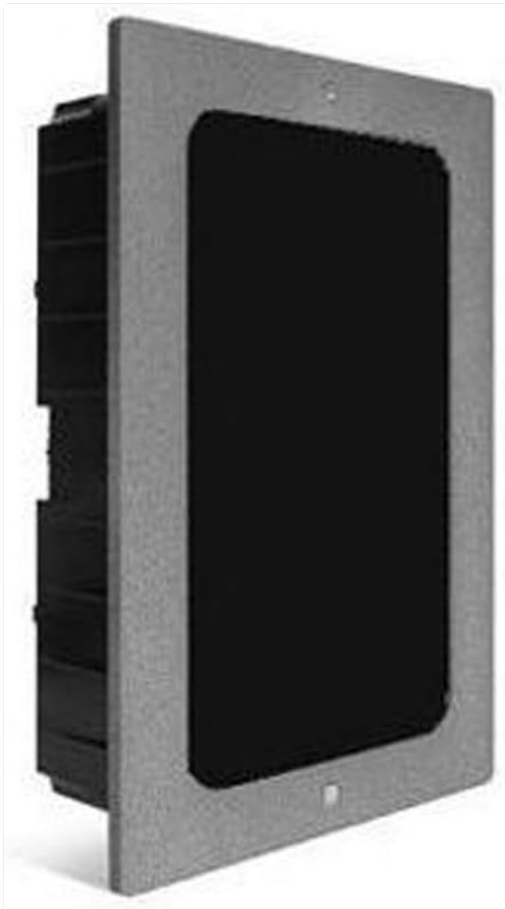
Figure 1: Front view of the Urmet Mikra Housing 1122/50, showing the gray aluminum frame and the black recessed area for audio kit installation. The housing is designed for flush mounting.
