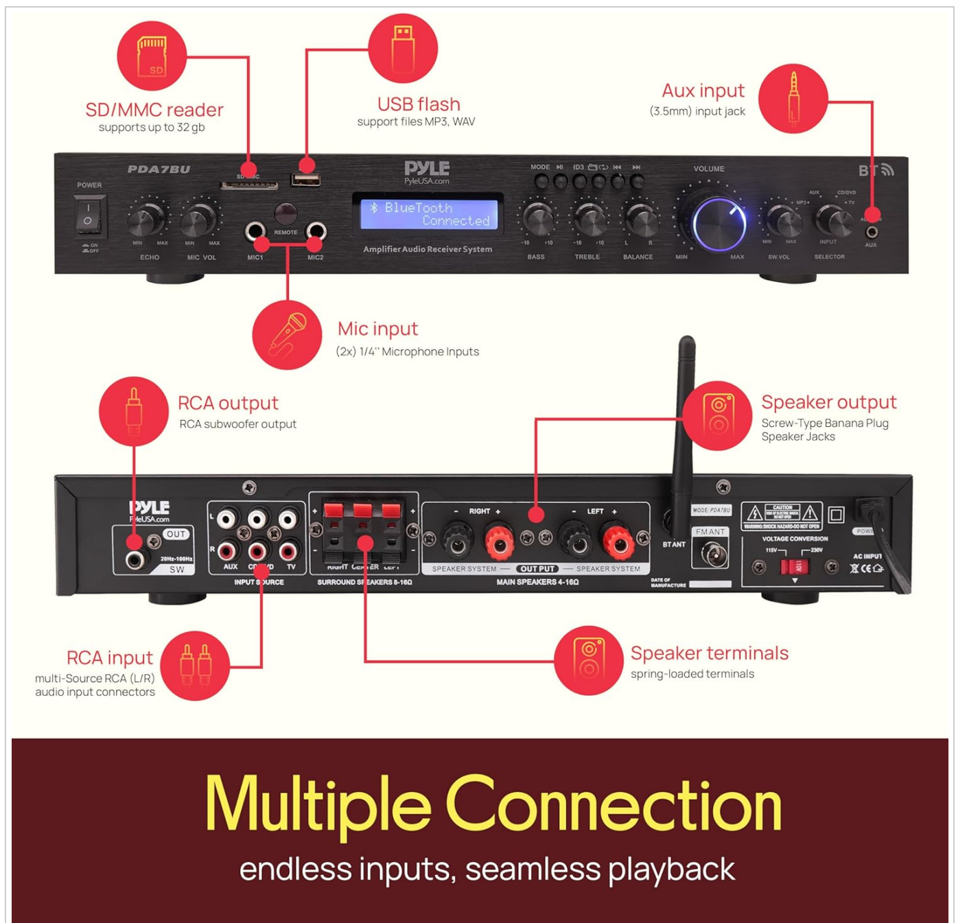
Image: Comprehensive diagram labeling all input and output connections on both the front and rear panels of the amplifier.
