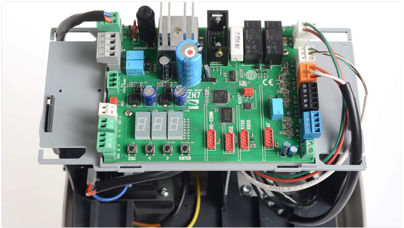
Image: Detailed view of the CAME BXV electronic control board, showing various terminals for connections and the display for configuration.
