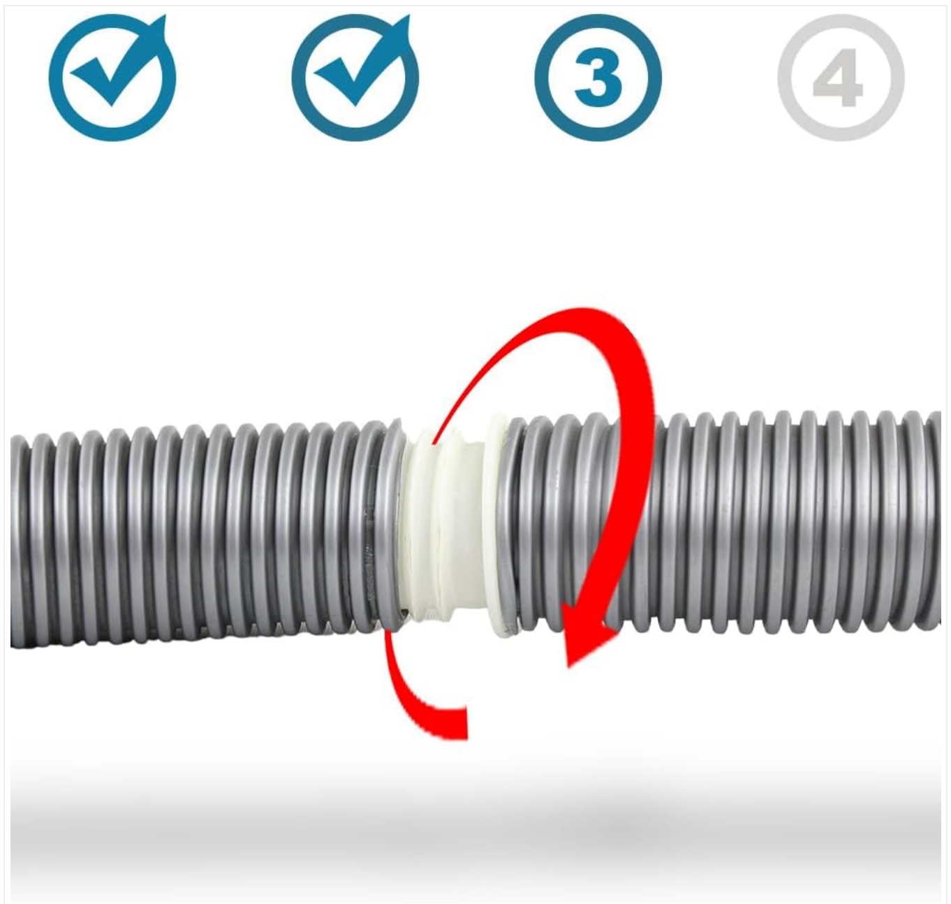
Figure 3: The repair piece being twisted into the hose, with arrows indicating the rotational movement for secure attachment.
