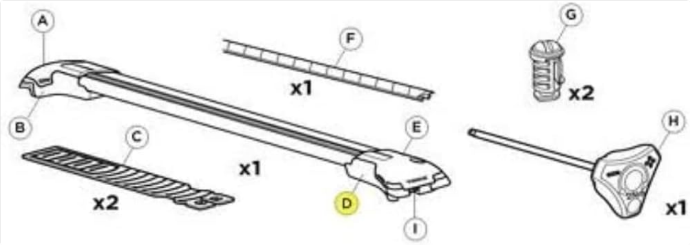
Image Description: This diagram illustrates the various components included with the THULE Edge Foot Railing LH 958. Key parts are labeled with letters A through I. These include the main roof bar assembly (A, B, E, I), rubber strips (C), a measuring strip (F), end caps (G), and a torque wrench (H). The main bar is shown with quantity 'x1', rubber strips 'x2', measuring strip 'x1', end caps 'x2', and torque wrench 'x1'. A circular highlight (D) indicates a specific point on the foot.
