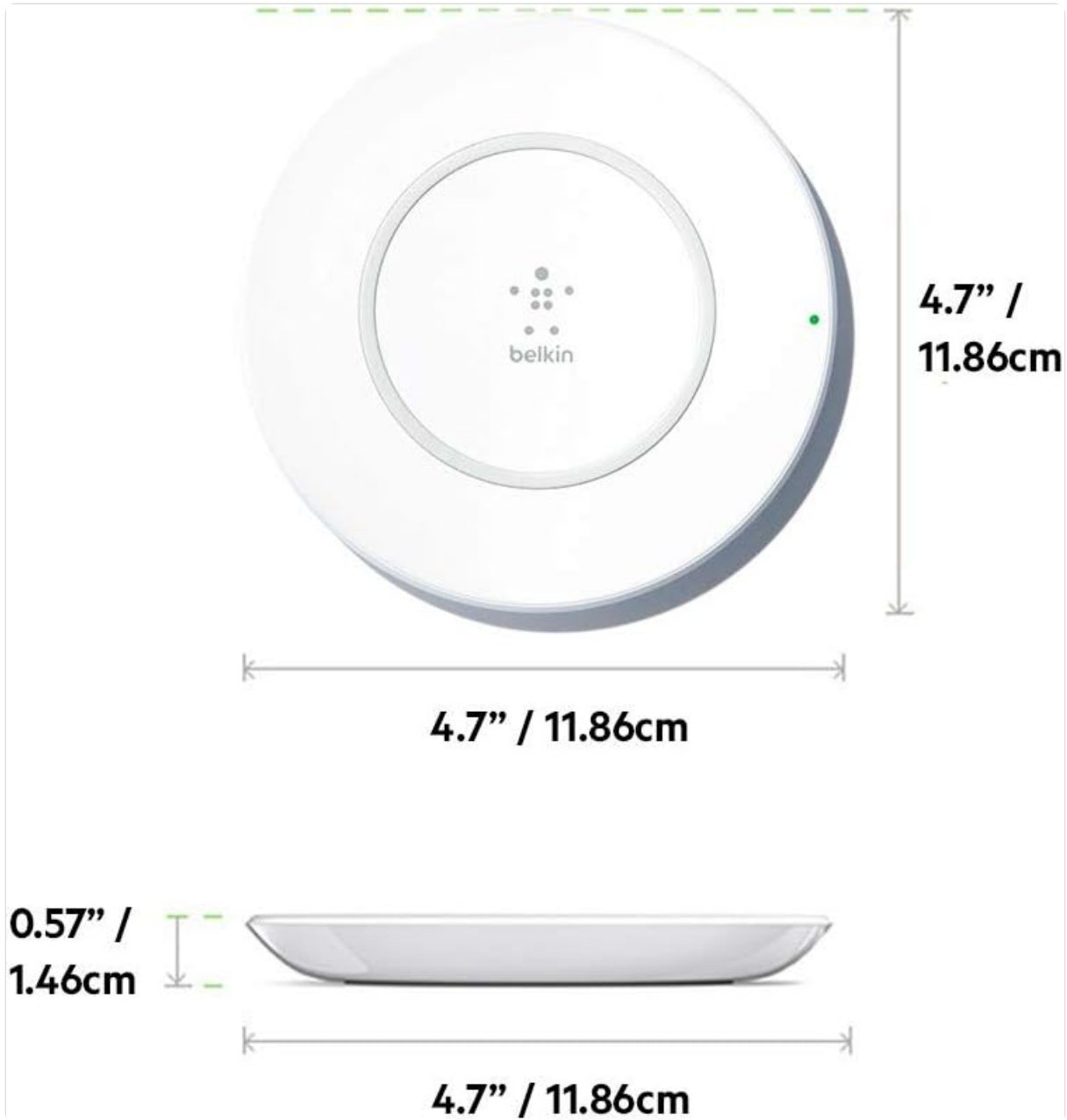
Image: A diagram illustrating the dimensions of the Belkin Quick Wireless Charging Pad, showing its compact and slim profile.
