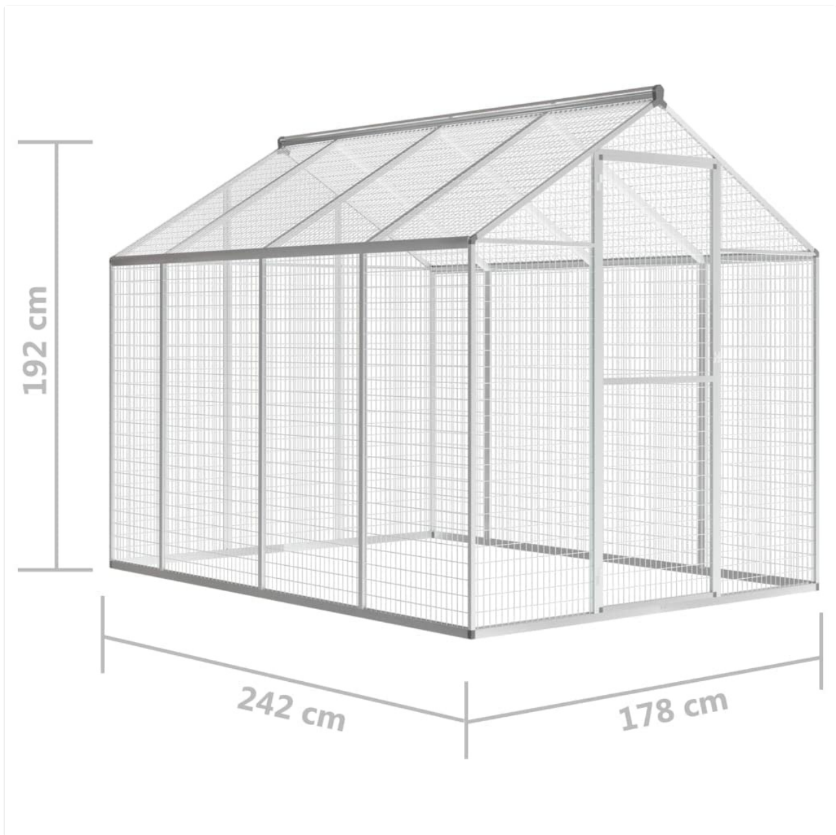
Figure 5.1: Aviary Dimensions.
