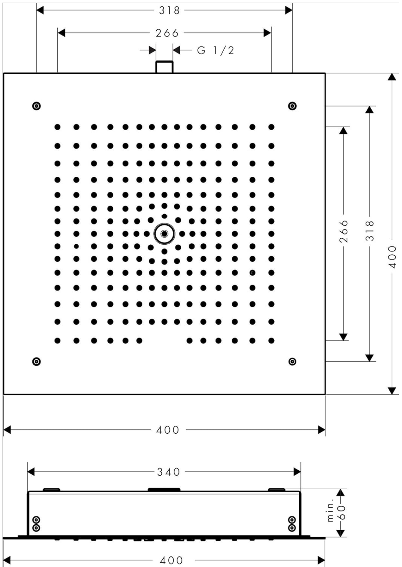
Figure 1: Technical drawing showing the dimensions (400x400mm) and connection points (G 1/2) for the hansgrohe Raindance E 400 1jet showerhead, including the minimum required installation depth of 60mm.
