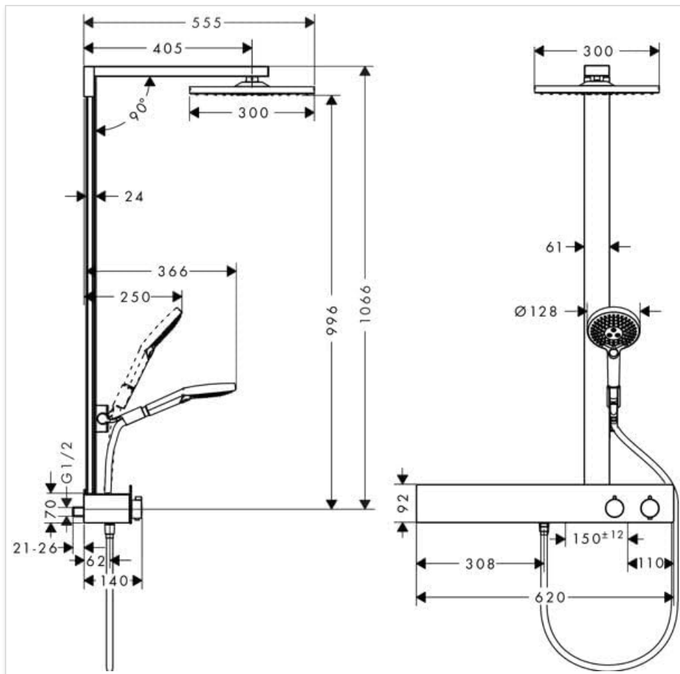
Figure 3.1: Technical drawing illustrating the dimensions and installation points for the hansgrohe Raindance E 300 Showerpipe. This diagram provides critical measurements in millimeters for the overhead shower, hand shower, riser, and thermostat unit, including water inlet positions and mounting distances.
