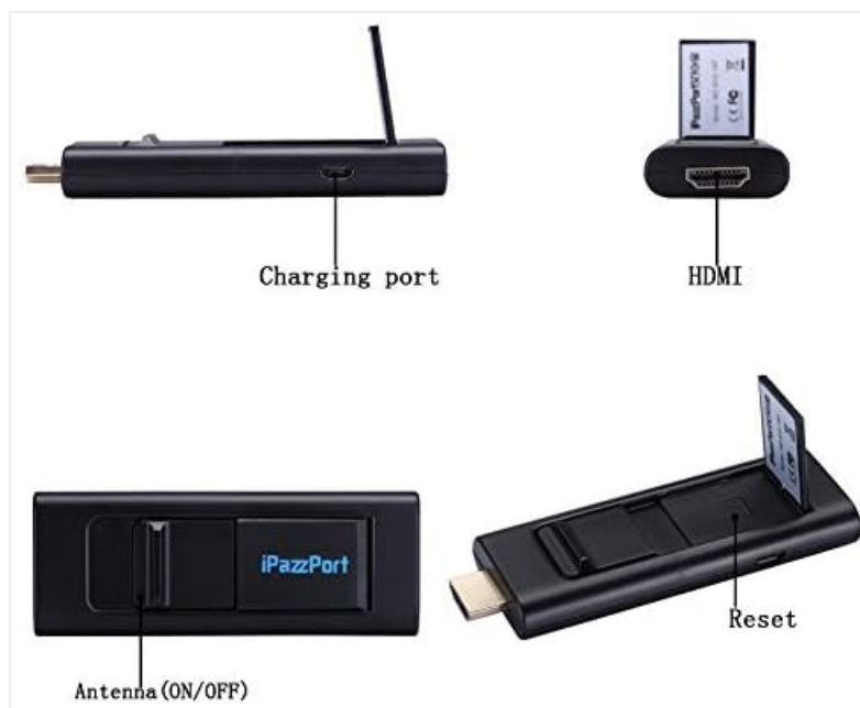
Image: Detailed view of the iPazzPort adapter showing the charging port, HDMI connector, and antenna switch.
