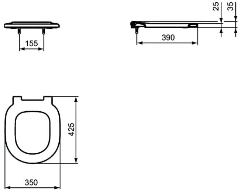
Image: Technical drawing showing key dimensions of the toilet seat.
