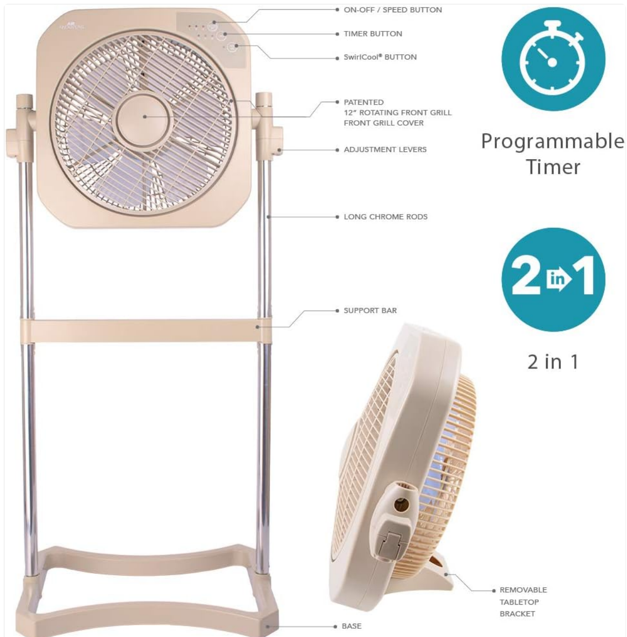
Figure 2: Fan Components Diagram
