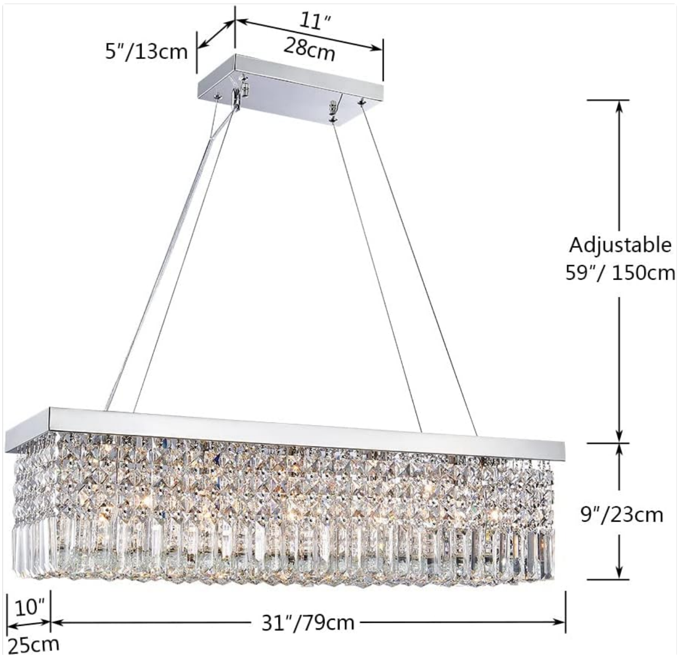
Figure 1: Chandelier Dimensions. This diagram illustrates the overall dimensions of the chandelier, including its length (31 inches), width (10 inches), fixture height (9 inches), and the adjustable chain length (up to 59 inches).
