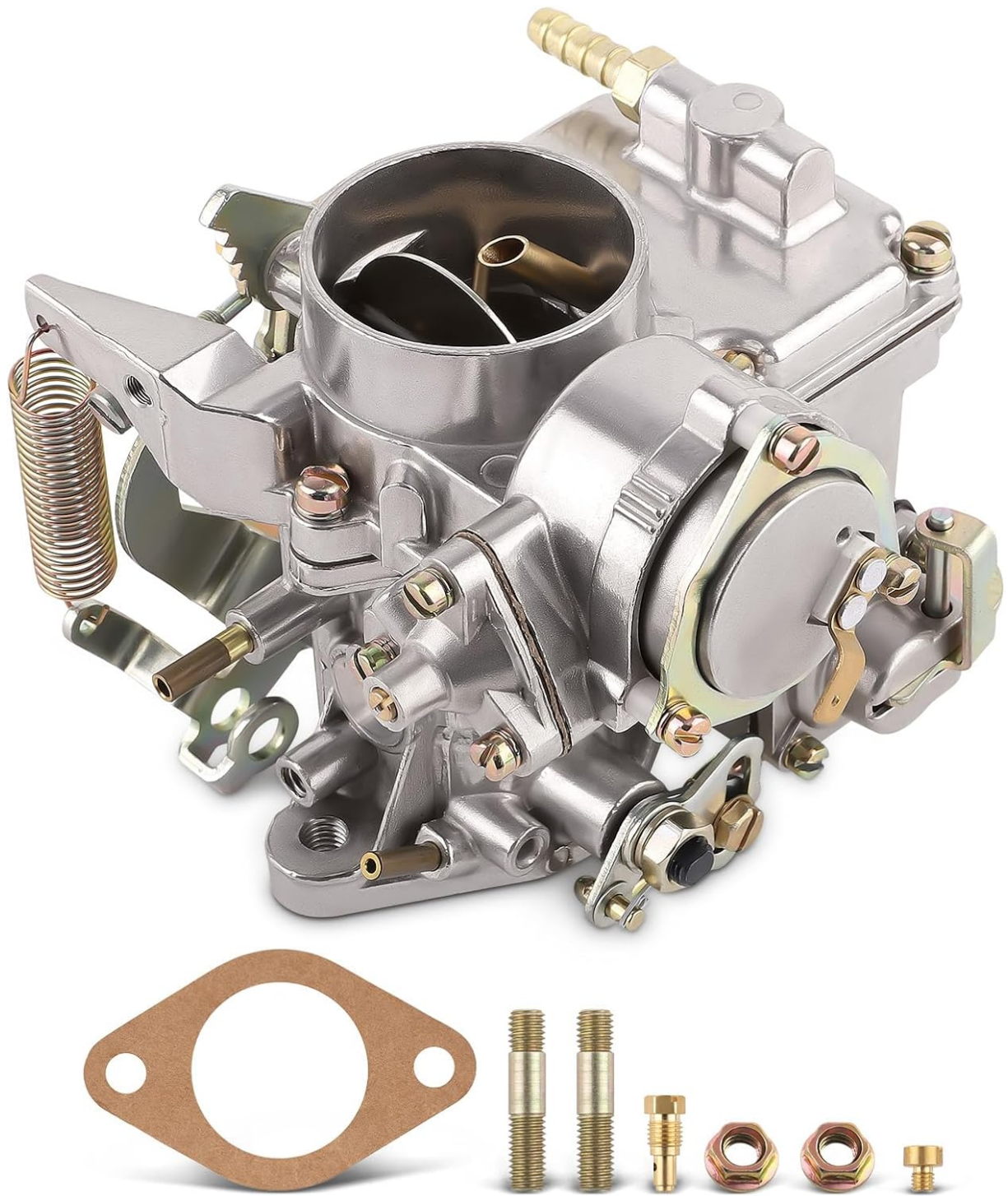
Figure 1: maXpeedingrods 34 PICT-3 Carburetor
