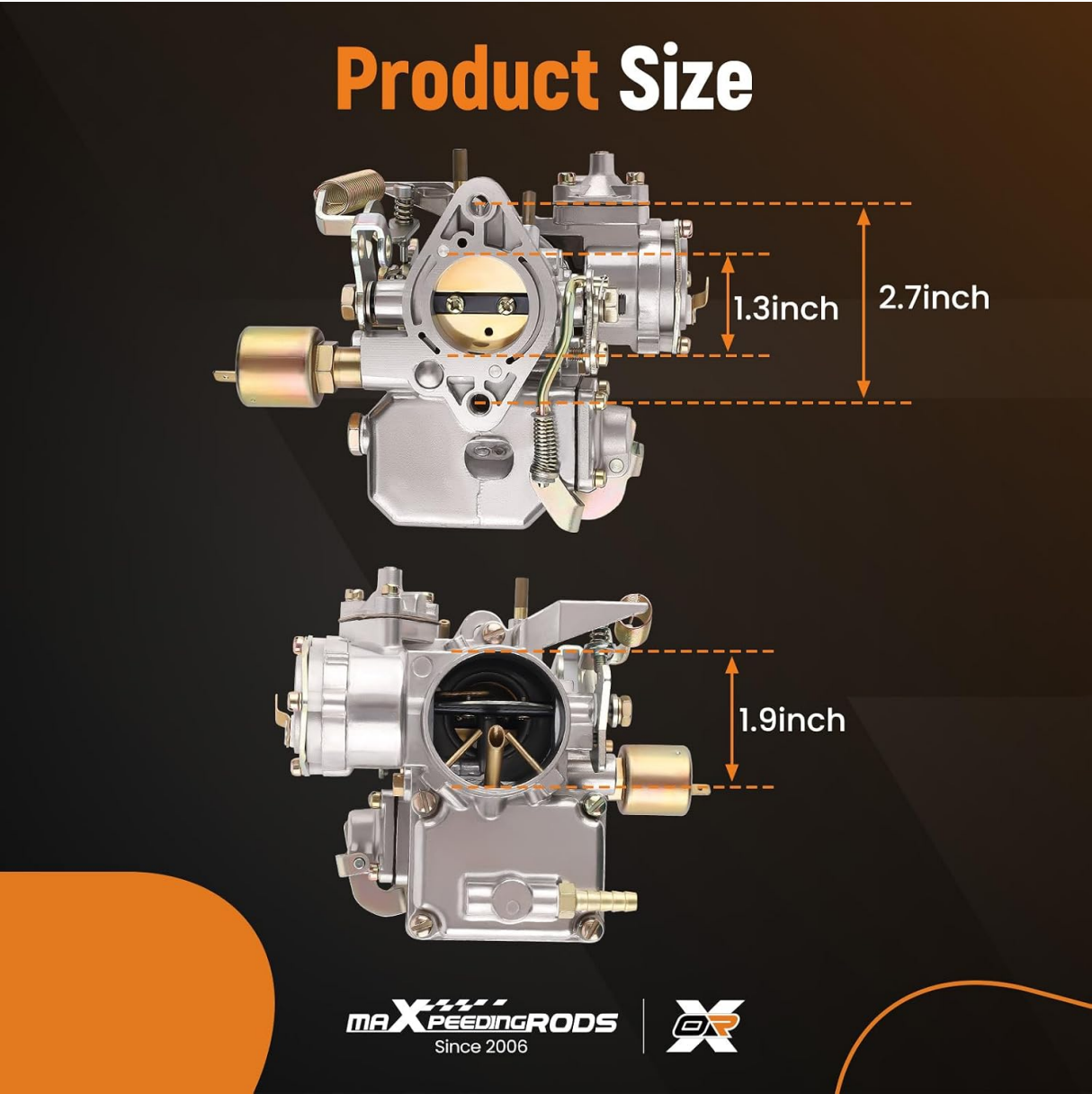
Figure 5: Product Dimensions
