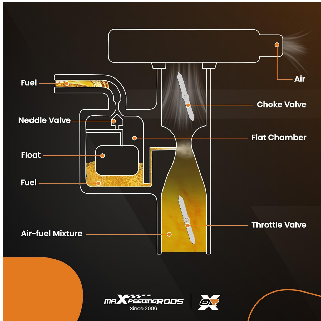
Figure 6: Basic Carburetor Function Diagram
