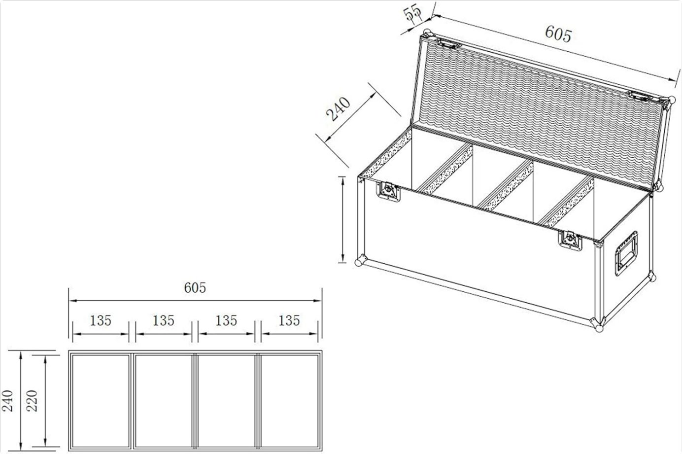
Figure 4: Technical drawing illustrating the dimensions of the lightmaXX TOUR CASE.
