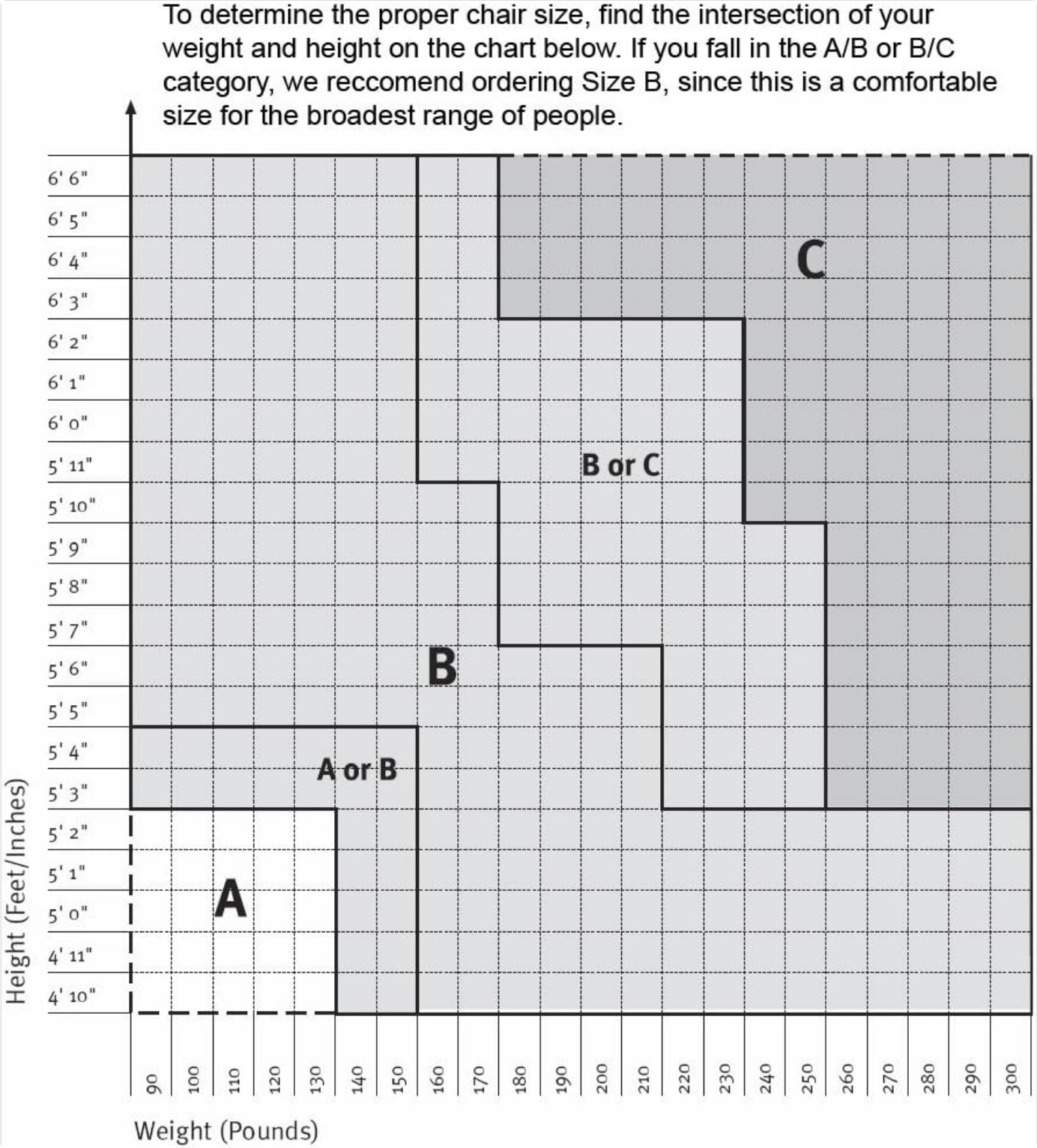
Figure 5: Size B (Medium) chair dimensions and recommended user range.
