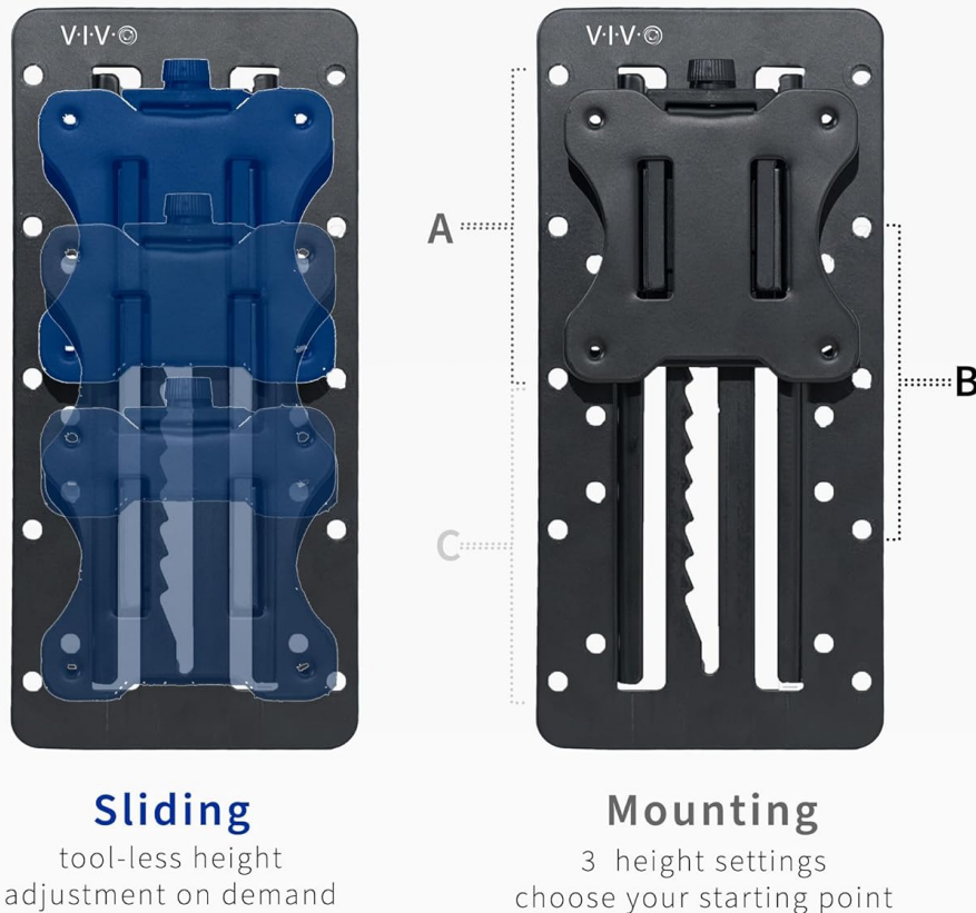
Figure 6: Diagram illustrating the 2-way height adjustment mechanism and mounting configurations.
