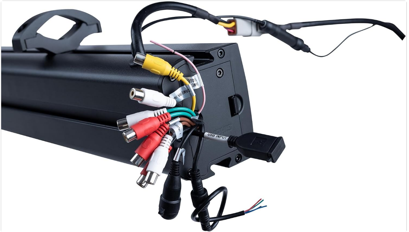
Figure 4: End cap removed, showing various input and output connections.
