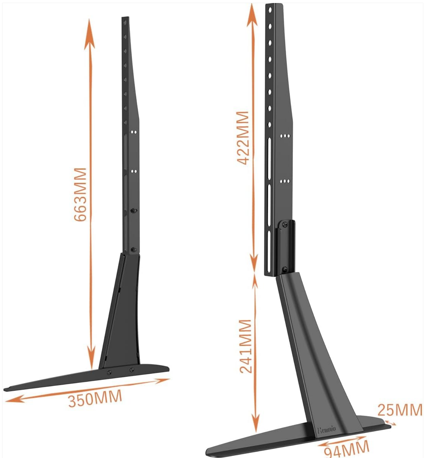
Image 4.1: Detailed dimensions of the stand components.
