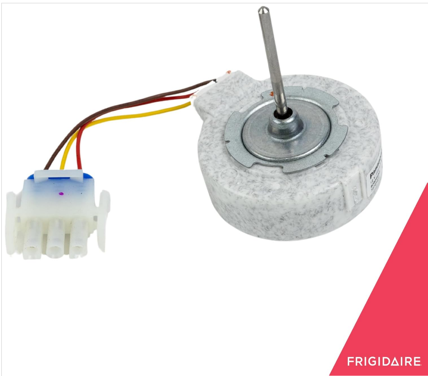
Image: An angled view of the Frigidaire 809069201 Evaporator Fan Motor, highlighting its compact design and the electrical connector.
