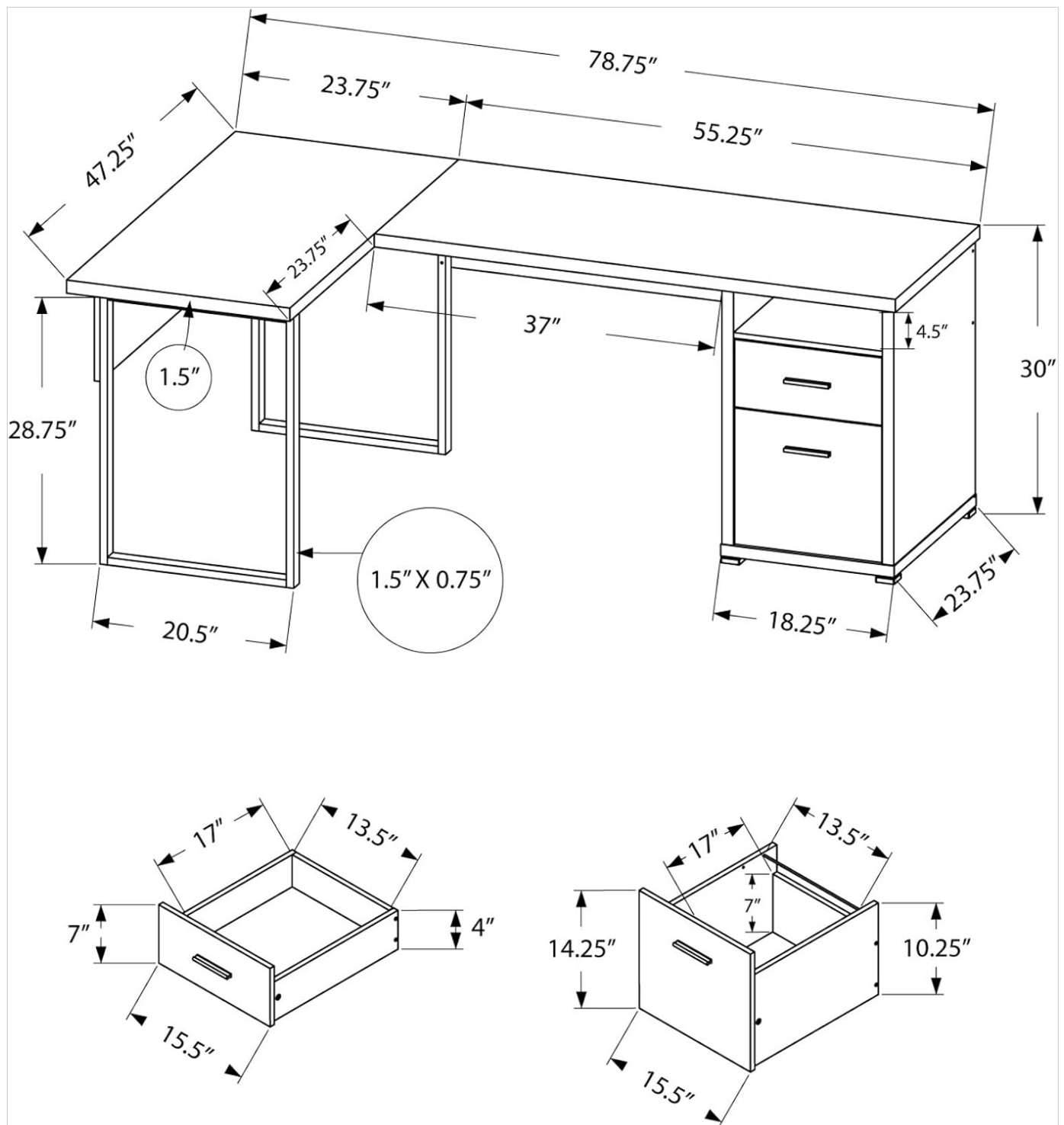
Figure 2: Dimensional diagram of the Monarch Specialties I 7257 L-Shaped Computer Desk, illustrating overall size and component measurements.
