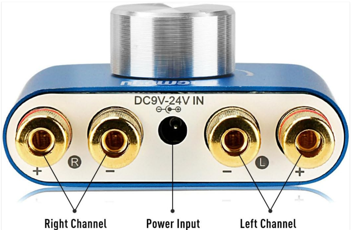
Image: A close-up of the amplifier's rear panel, showing the DC 9V-24V power input jack and the speaker output terminals for the left and right channels, compatible with both bare wire and banana plugs.
