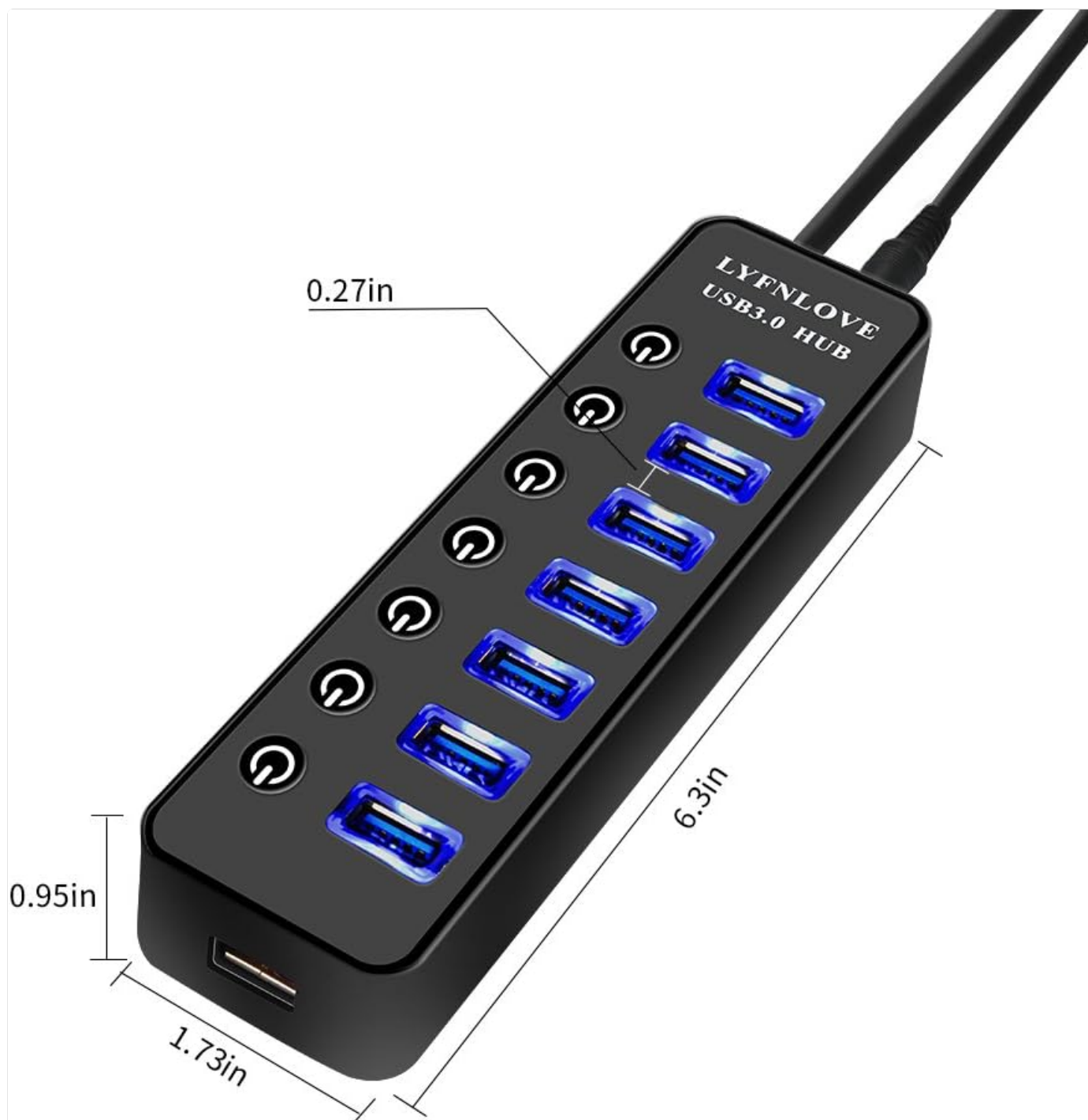
Image 7.1: Image displaying the dimensions of the LYFNLOVE USB 3.0 Hub, showing its length (6.3 inches), width (1.73 inches), and height (0.95 inches).
