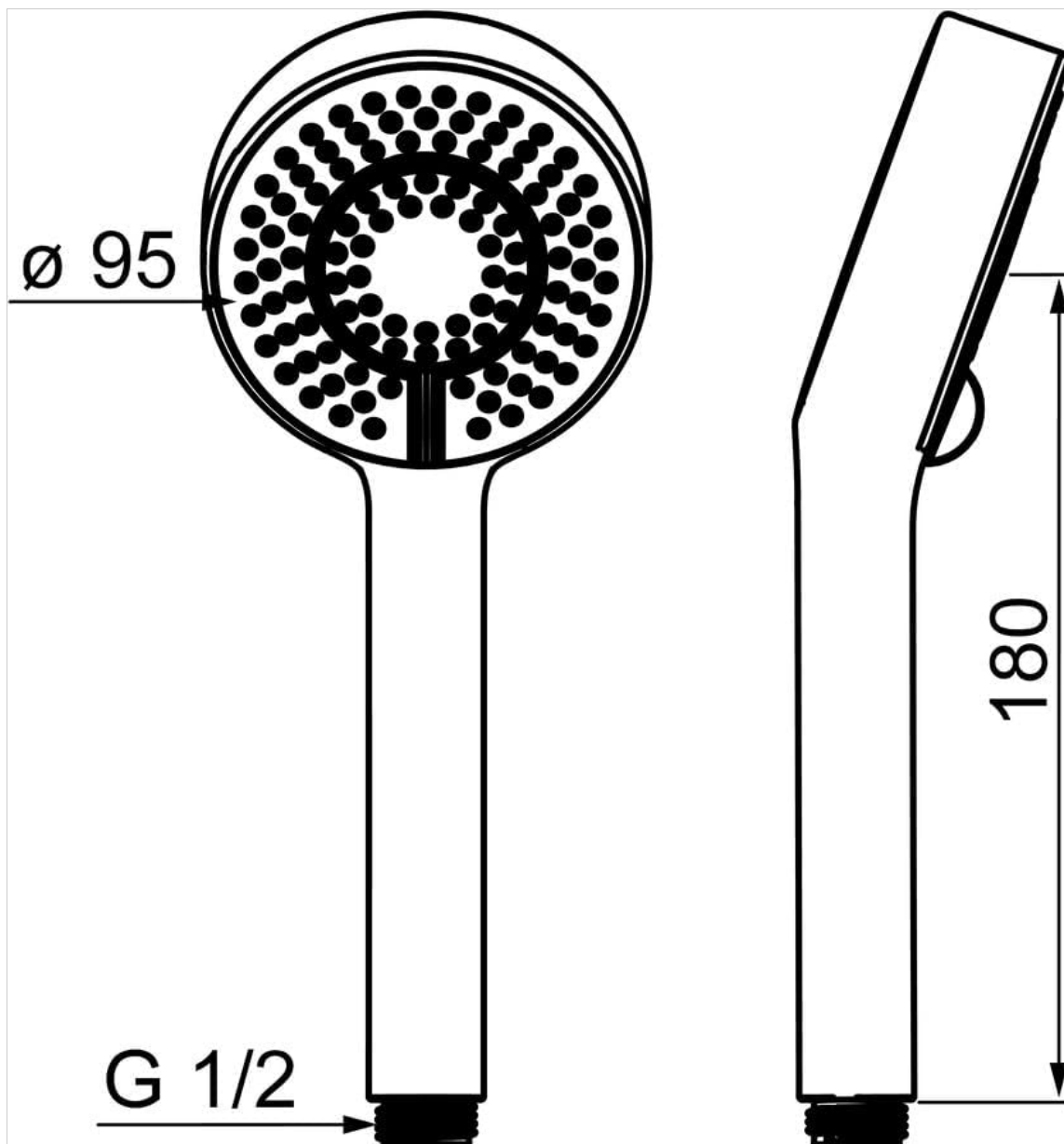
Image 8.1: Technical drawing illustrating the dimensions (diameter 95mm, length 180mm) and G 1/2 hose connection of the Hansa Basic Jet shower head.
