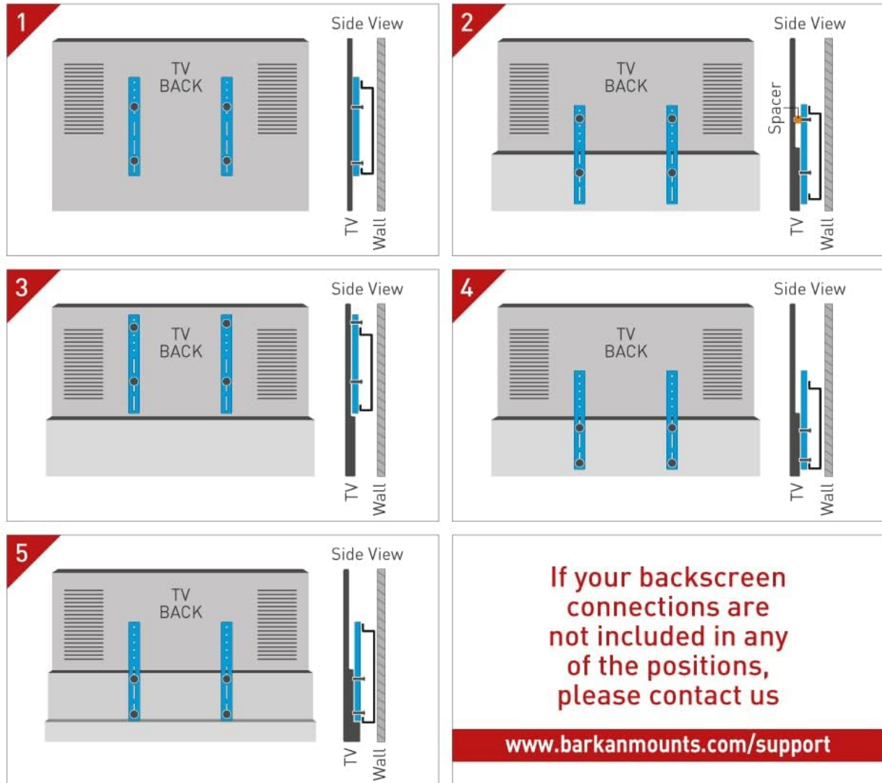
Figure 3.3: Different backscreen connection positioning options for the vertical rails.
