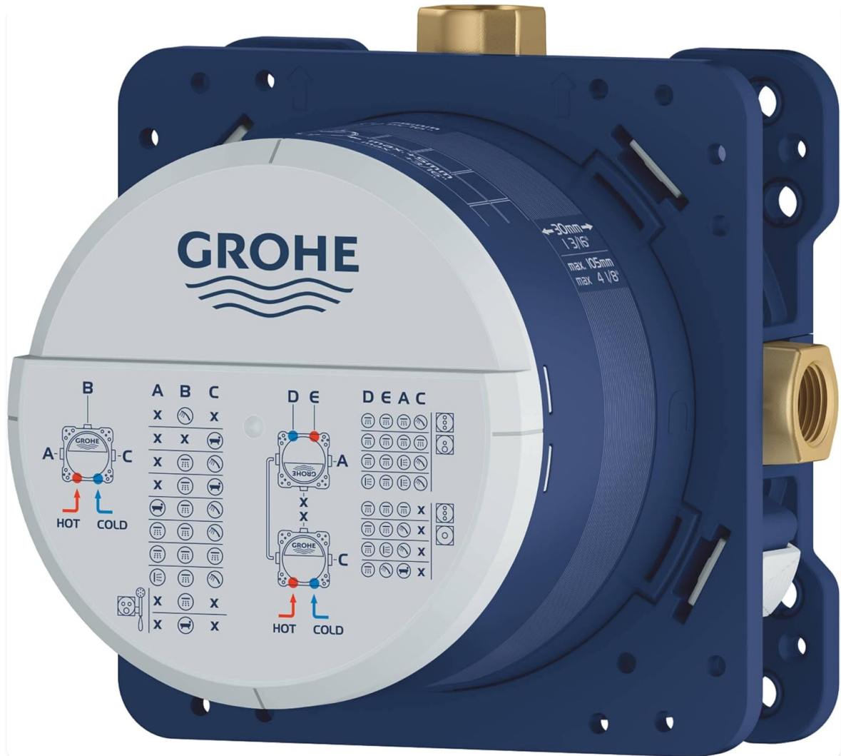
Figure 6: The Smartbox with its protective cover displaying the piping matrix for various configurations.
