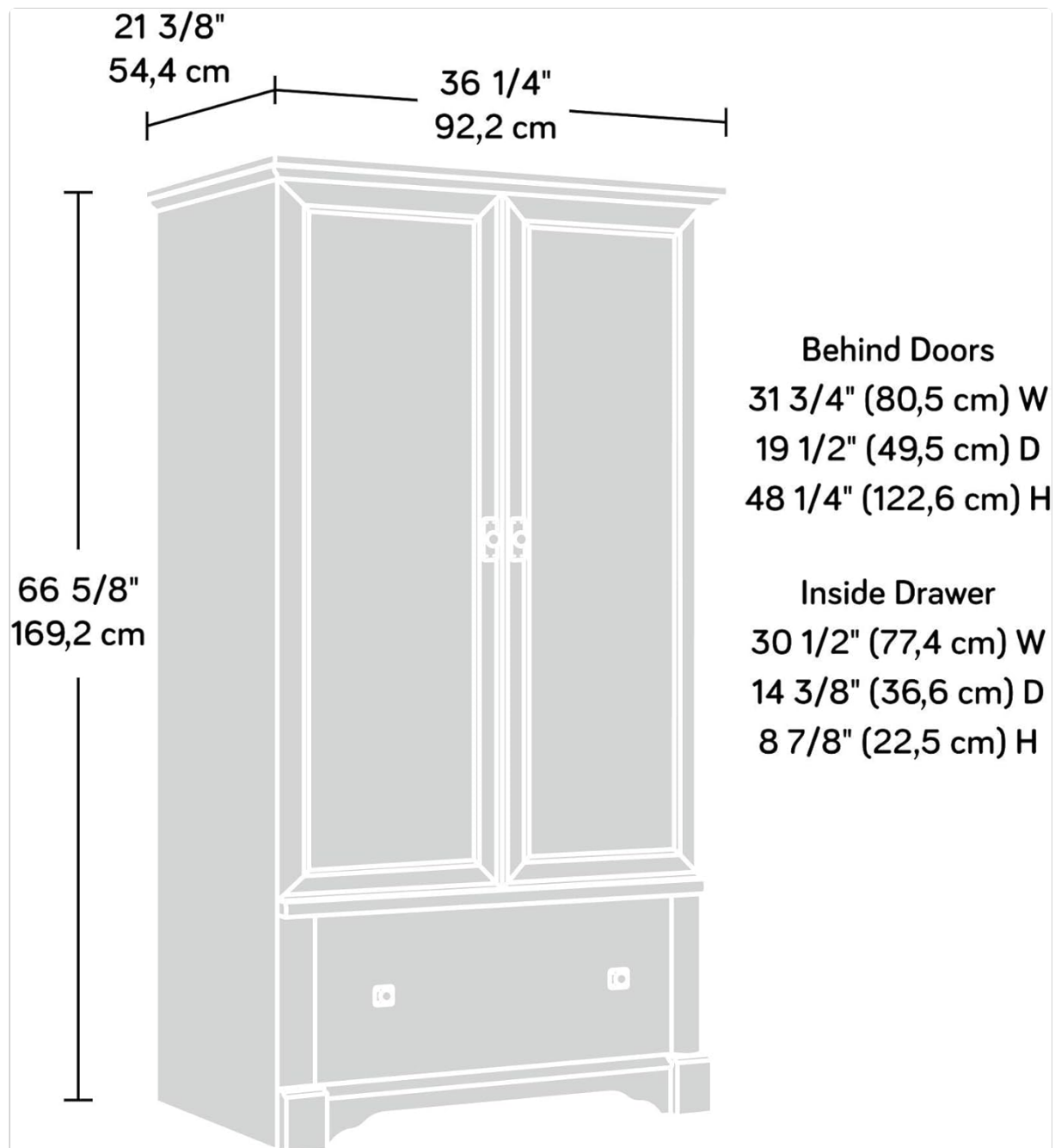
Figure 2: Dimensional diagram of the armoire, indicating overall height, width, depth, and internal storage measurements.
