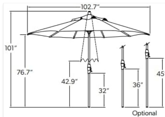
Figure 2: Technical diagram illustrating the dimensions of the 9ft Octagonal Patio Umbrella, including height and canopy width.
