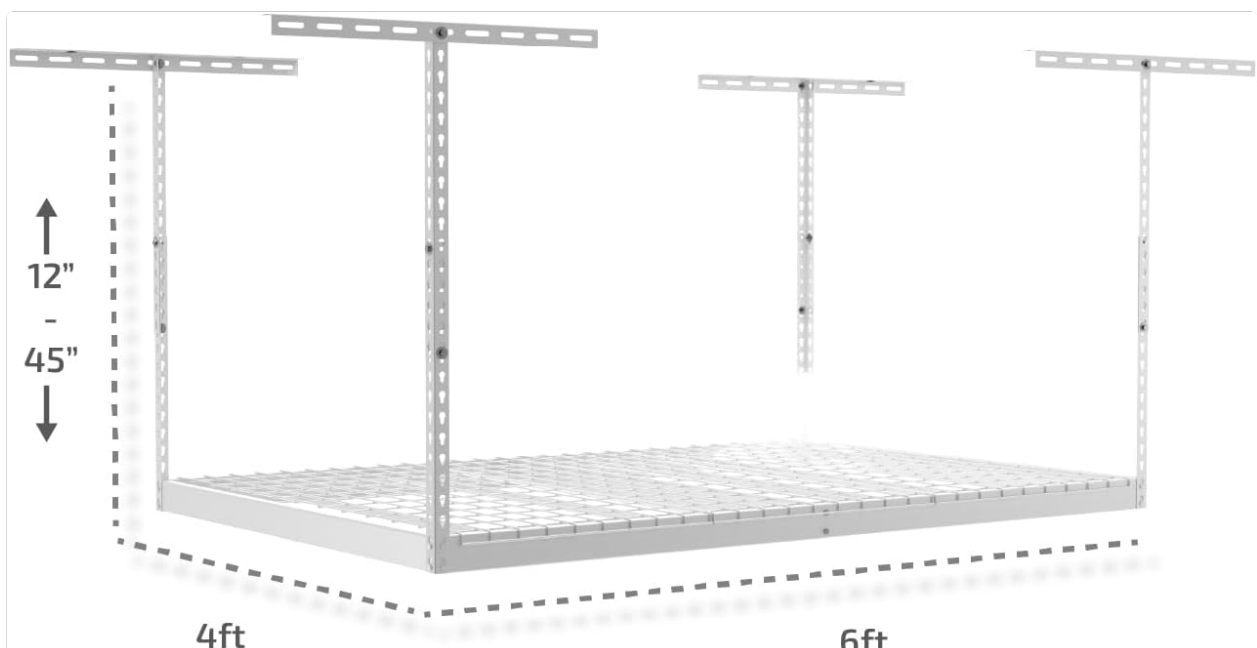
Figure 4.1: Dimensions and adjustable height range of the SafeRacks 4x6 unit.
