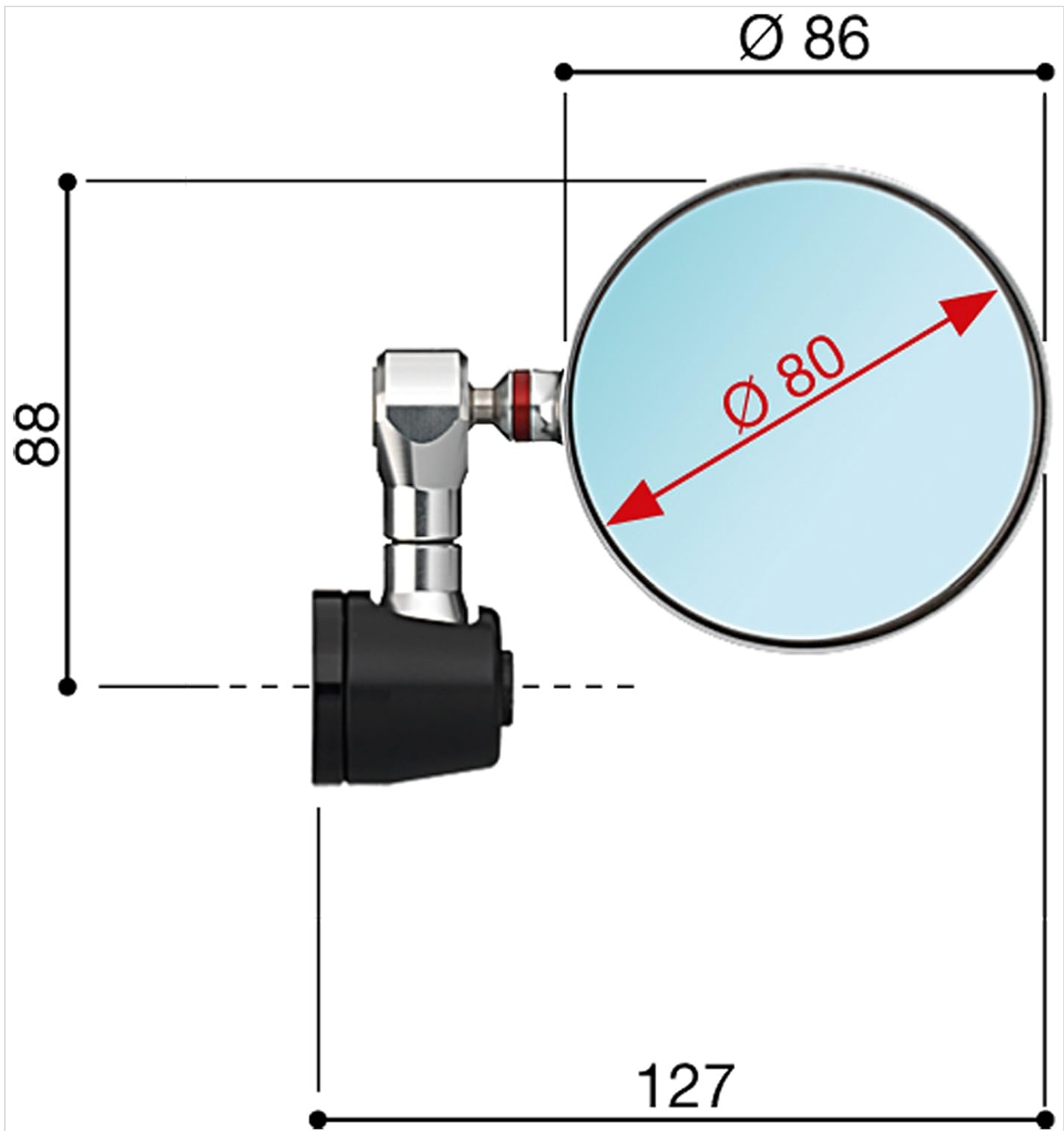
Figure 8.1: Detailed technical drawing showing the dimensions of the Rizoma Spy R 80 Mirror and its adapter.
