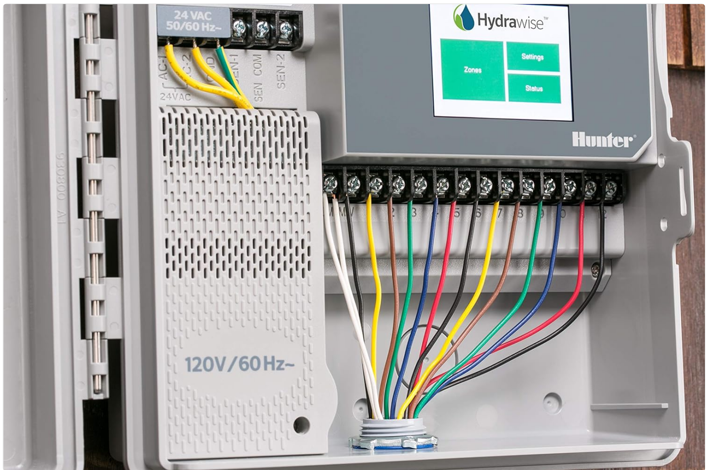
Figure 2: Detailed view of the wiring compartment, showing the connection points for individual zone wires (numbered terminals) and the common wire (COM). The AC power input is also visible at the top left.
