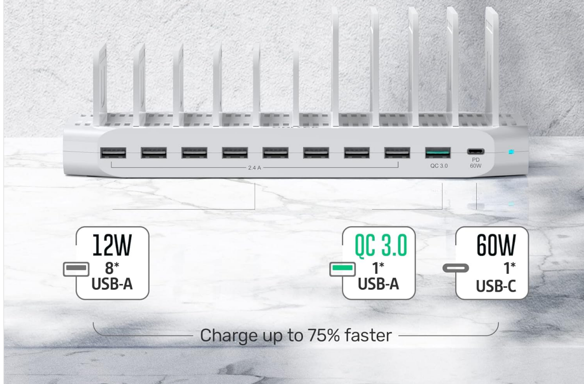
Figure 2.1: Overview of the charging station's ports and their respective power outputs, highlighting the 160W total power. This image displays the various USB-A and USB-C ports, along with their wattage capabilities, such as 12W for 8 USB-A ports, 18W for 1 QC 3.0 USB-A port, and 60W for 1 USB-C port.
