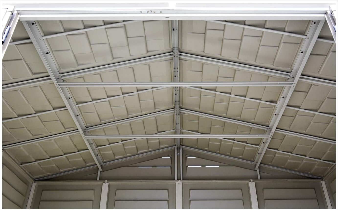
Figure 5: Roof structure detail
