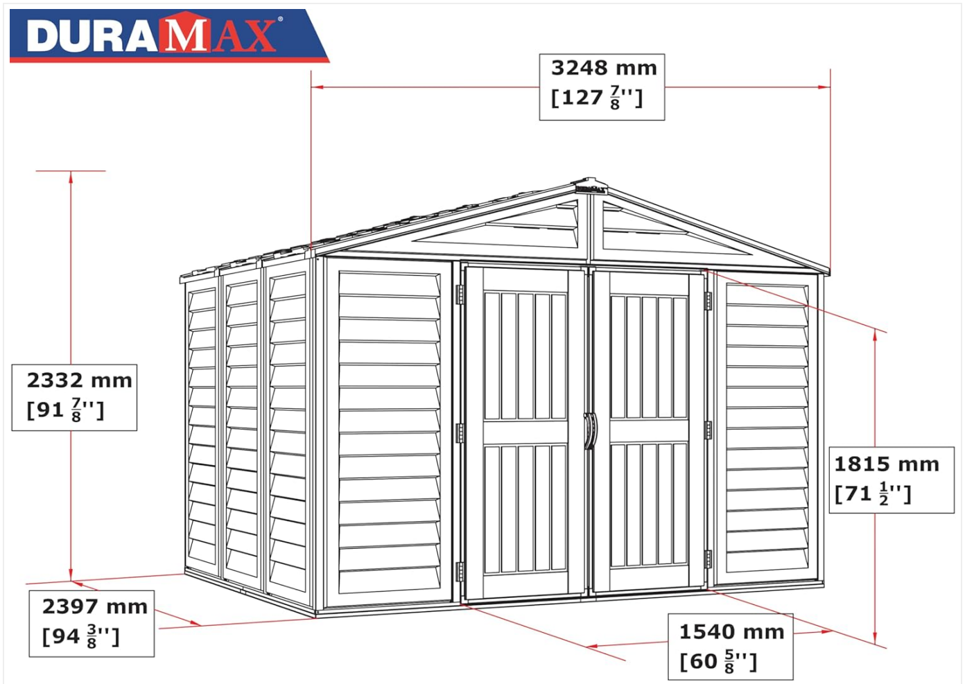
Figure 6: Shed dimensions overview
