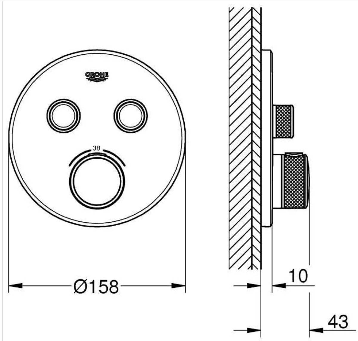
Figure 2: Technical diagram illustrating the dimensions and concealed installation requirements for the GROHE Grohtherm SmartControl Thermostat, including the wall rosette and connection points.
