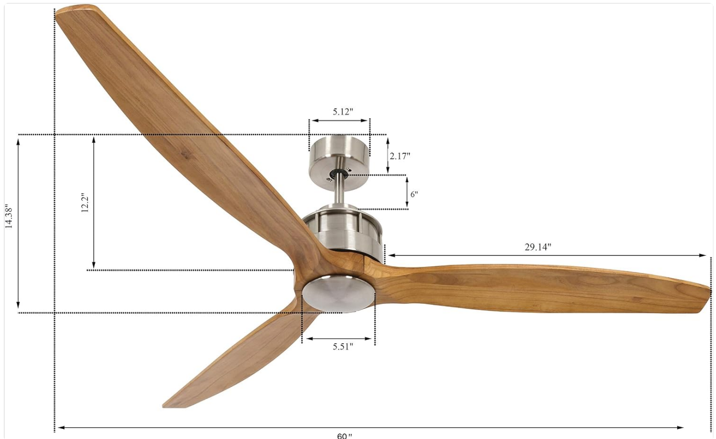
Figure 2.1: Fan Dimensions for Installation Planning
