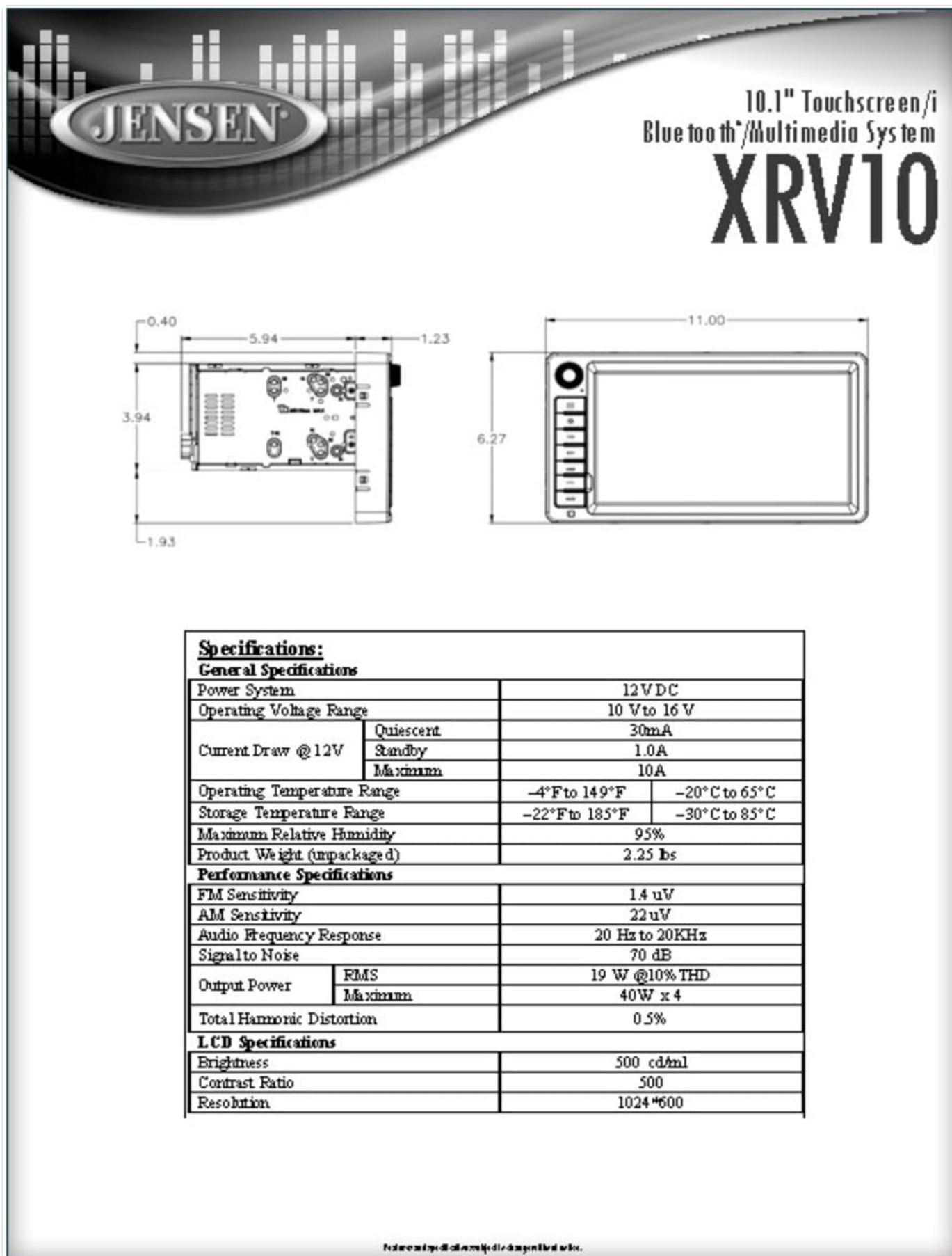
Figure 3: Technical specifications and dimensional drawing of the Jensen XRV10 multimedia system.
