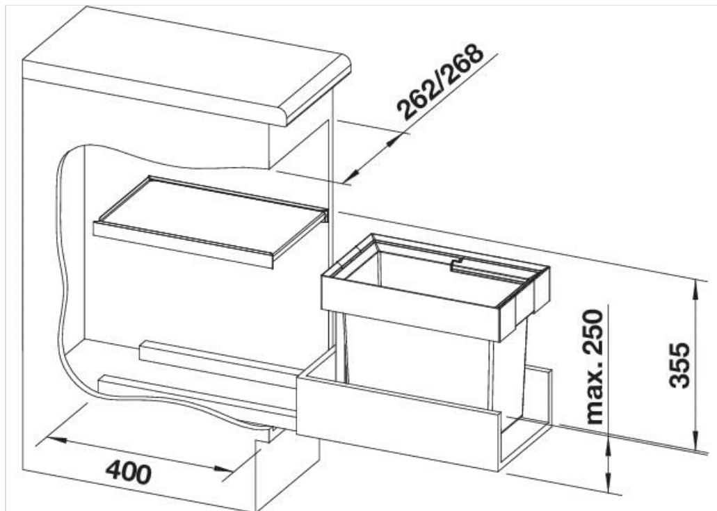
Image: Technical diagram illustrating the installation of the BLANCO Flexon II system within a base cabinet drawer, showing critical dimensions for depth (400 mm), height (355 mm), and width (262/268 mm).
