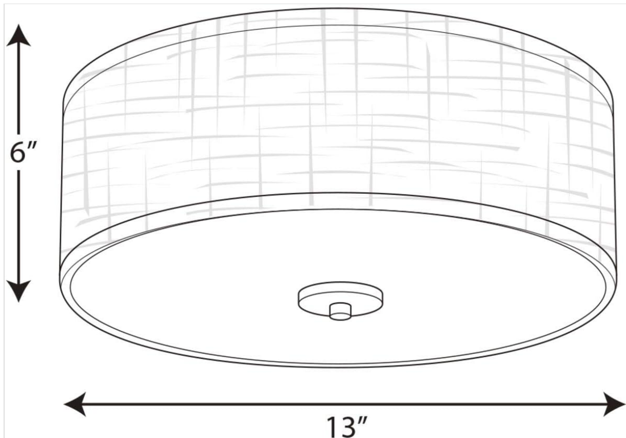
Figure 2: Dimensional drawing of the Inspire LED Flush Mount, showing a 13-inch diameter and 6-inch height.
