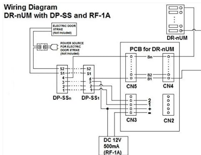
Figure 3: Wiring Diagram for DR-nUM (DR-4UM) with DP-SS and RF-1A
