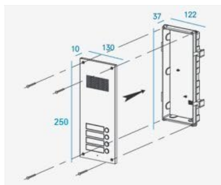
Figure 2: Installation Dimensions (Measurements in mm)
