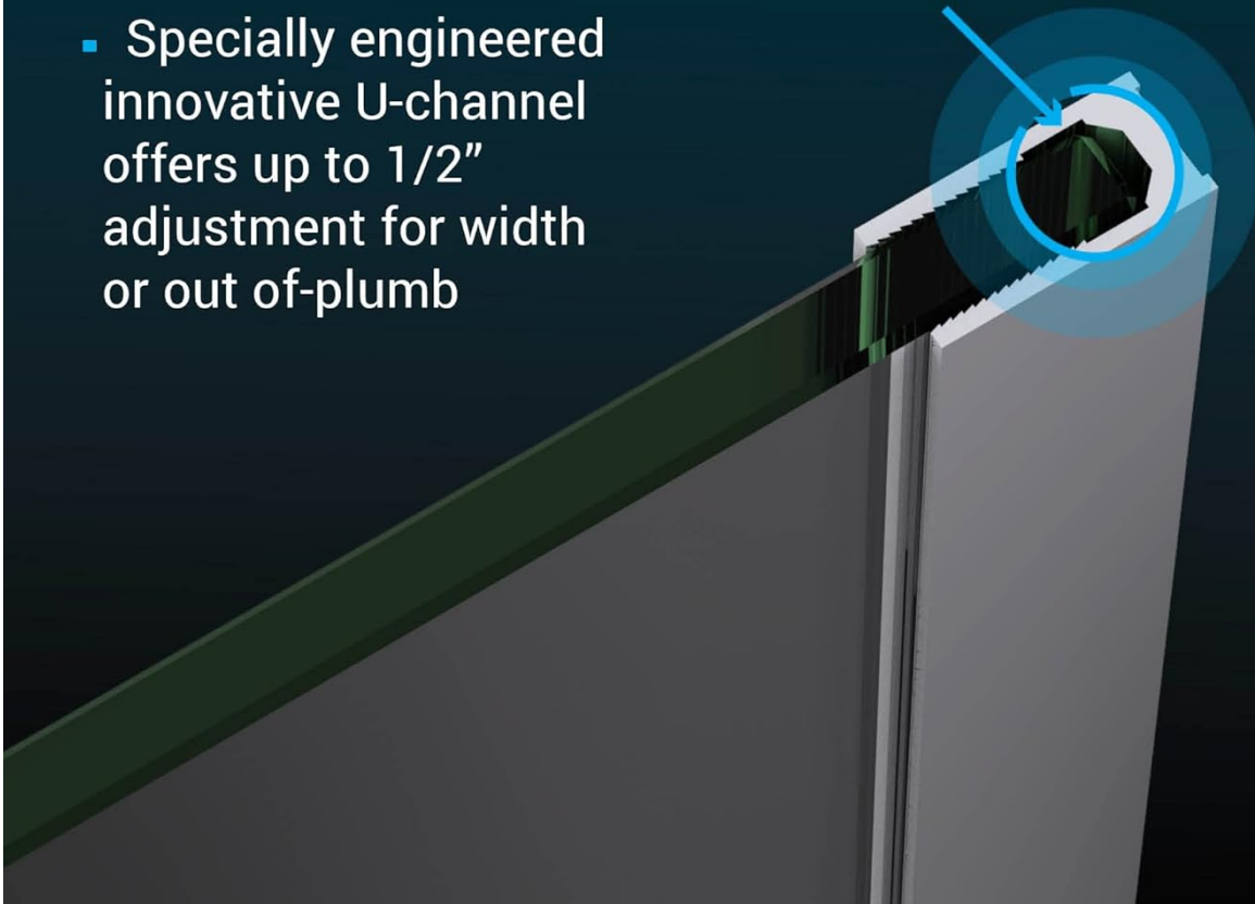
Figure 4: Detail of the U-channel providing out-of-plumb adjustment.
